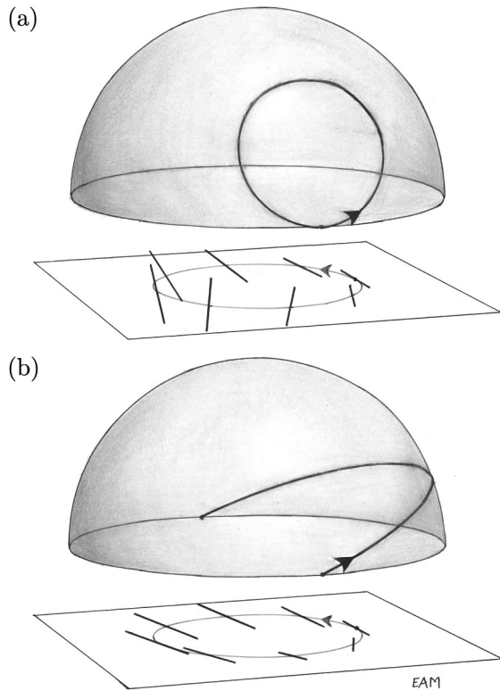
FIG. 3. The GSM for the three-dimensional nematic is the real projective plane \mathbb{RP}^2 . Below each hemisphere which represents \mathbb{RP}^2 we draw the path in the sample and the corresponding director at each point, with the arrows on the two curves denoting corresponding points and orientations. Any measurement around a closed loop in the sample can be mapped to a path in \mathbb{RP}^2 which belongs to one of two homotopy classes: (a) trivial and (b) nontrivial. In other words, \pi_1(\mathbb{RP}^2) = \mathbb{Z}_2 .
