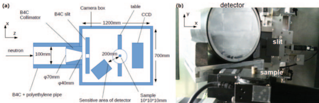
Fig. 2. – Experimental setup of diffraction measurement in RANS.
