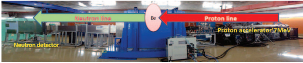
Fig. 1. – RANS entire view.
